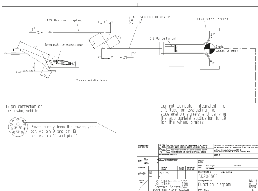
Figure: Diagram of the retrofittable ETS brake system
